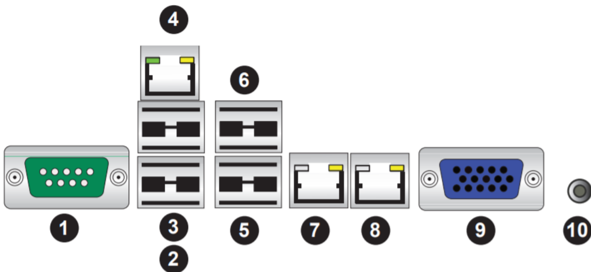
Figure 5-1. Rear I/O Ports
